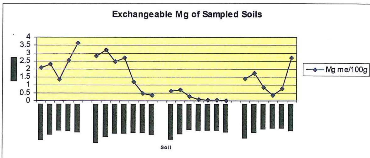
Figure 5.4. Exchangeable Mg of sampled soils (me/100g).
