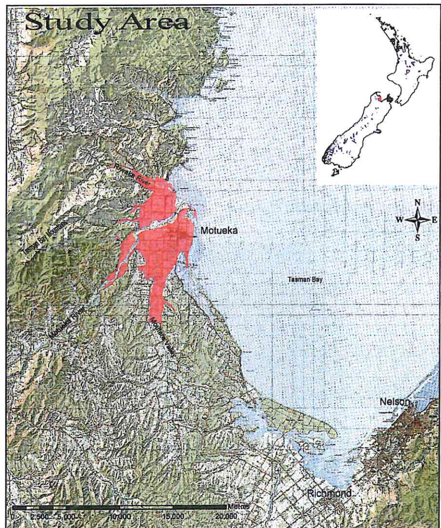
Figure 1. Location of the Motueka soil map.
