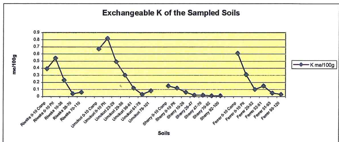
Figure 5.2. Exchangeable K of sampled soils (me/100g).
