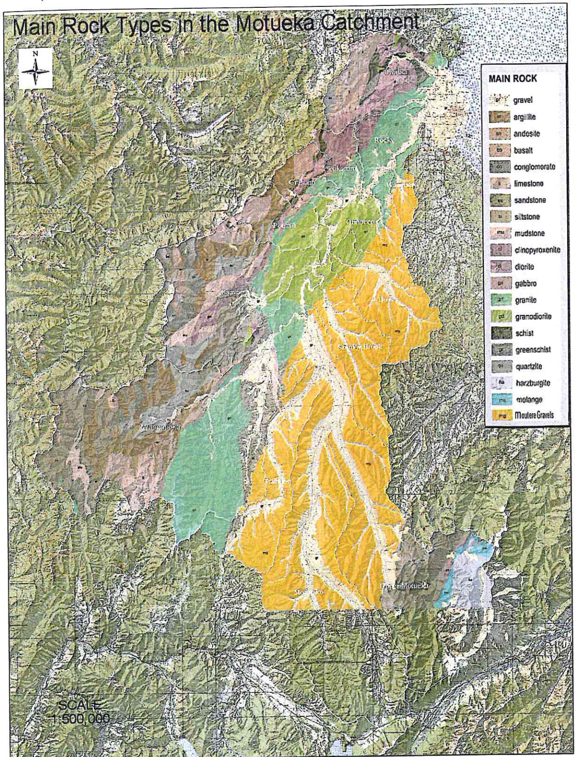
Figure 2.2. Geology of the Motueka and Riwaka Catchments ( adapted from Rattenbury et al., 1998 ).
