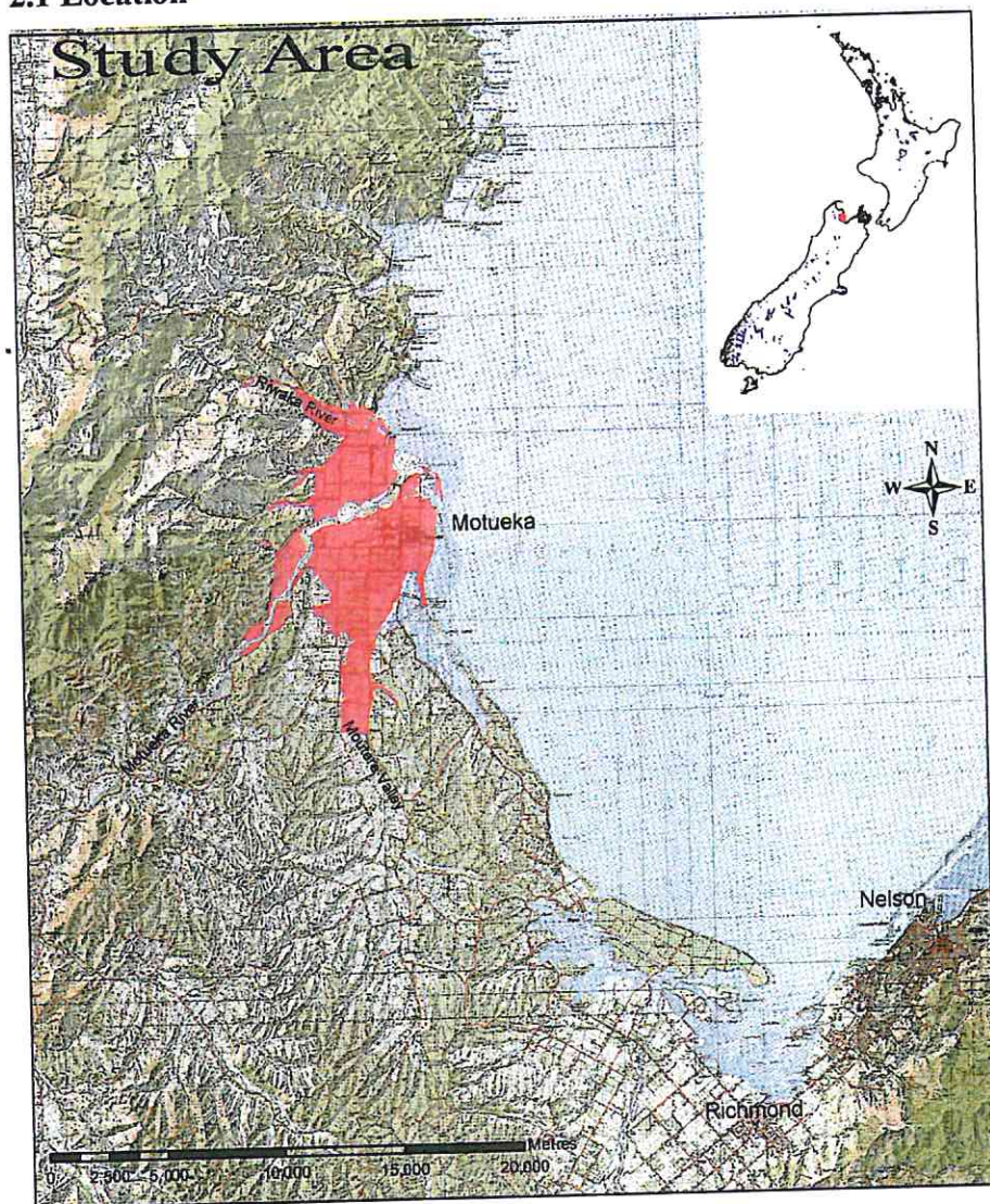
Figure 2.1. Extent of the existing soil map.
