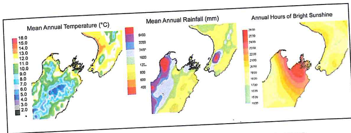
Figure 2.3. Climate summary of the region (adapted from Mackintosh, 2001).
