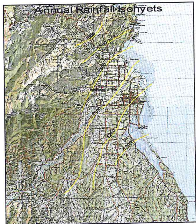
Figure 2.4. Rainfall Isohyets for the study area.
