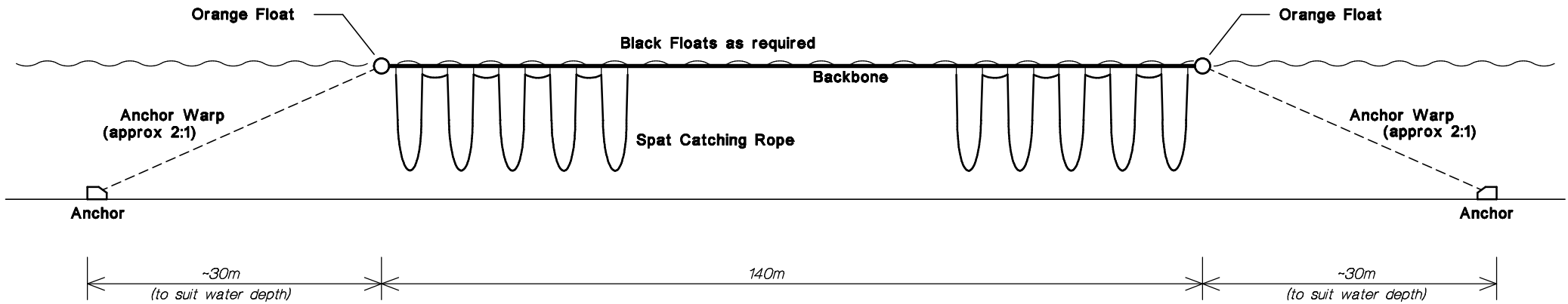
Longline Elevation (Not to Scale)
